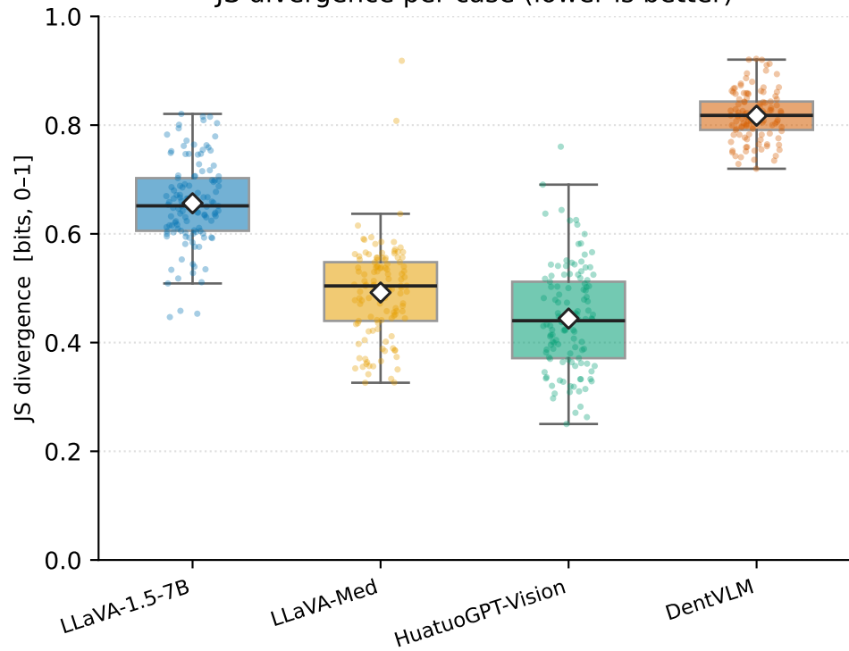
JS divergence per case (lower is better)
